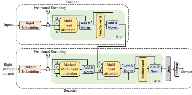
Figure 9: Transformer architecture.
