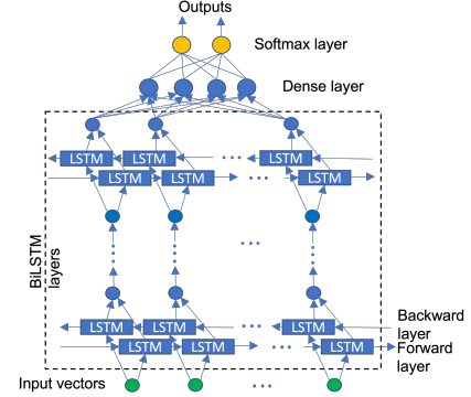
Figure 8: BiLSTM architecture.
